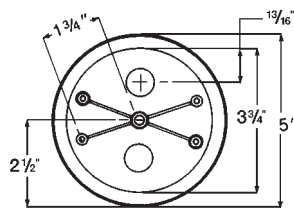
Surface Mount Wiring Box For Model 101
